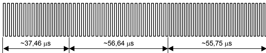
Figure 17 — End of frame when using two subcarriers
